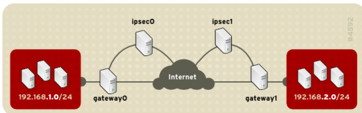
Figure 2.12. Network-to-Network IPsec
